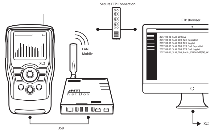
Remote Access to XL2-TA Sound Level Meter
